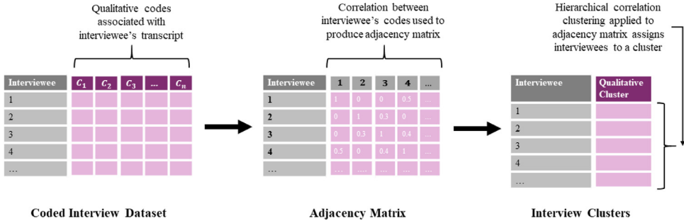
Fig. 4. Schematic of interview coding clustering process. Coded interview table is transformed into an adjacency matrix by calculating correlation between respondents. This adjacency matrix is then clustered to assign interviewees to respective clusters.
