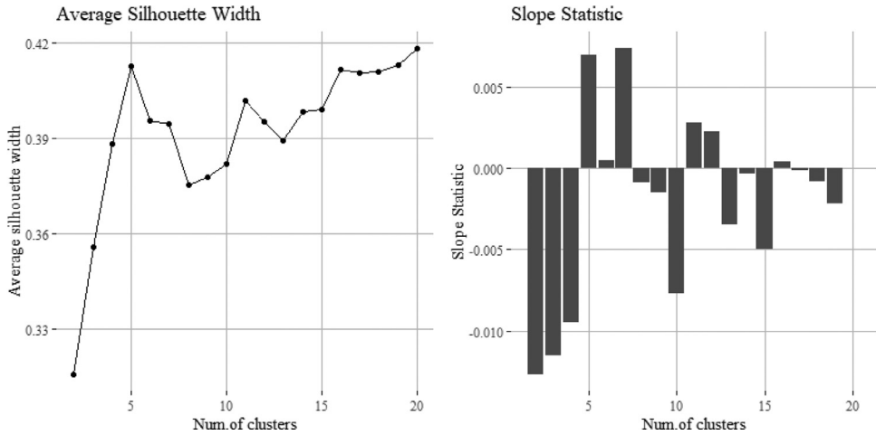
Fig. 3. Example of use of Silhouette Width and Slope Statistic to determine optimal number of clusters for a sample of households in Bangalore. Note how while there are maxima on the silhouette width plot at 5 and 16 the slope statistic indicates 5 as preferable.
