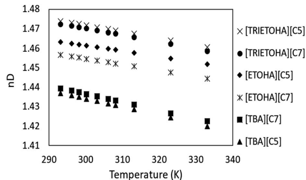
Fig. 5 The RI plot for APILs at temperature range 293.15–333.15 K.
