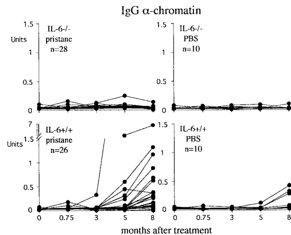
Figure 2. IgG antichromatin antibody ELISA. Serial serum samples from all pristane- or PBS-treated mice were analyzed at a dilution of 1:500 for IgG anti-chromatin antibodies by ELISA. Levels of IgG antichromatin are expressed in units × 10 6 (see Materials and Methods).
