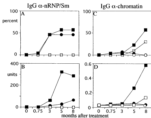
Figure 3. Anti-nRNP/Sm and anti-chromatin antibody ELISAs. Sera from pristane treated IL-6 -/- ( n = 28 , ●) or IL-6 +/+ ( n = 26 , ■) mice and from PBS-treated IL-6 -/- ( n = 10 , ○) or IL-6 +/+ ( n = 10 , □) mice 0–8 mo after treatment were tested for anti-nRNP/Sm (A and B) and anti-chromatin (C and D) antibodies by ELISA. (Top) Frequencies (%) of sera containing IgG anti-nRNP/Sm (A) or anti-chromatin (B) autoantibodies (defined as >3 SDs above the mean of negative controls). (Bottom) Levels of anti-nRNP/Sm (B) or anti-chromatin (D) autoantibodies (in units). Data represent the mean of all animals in each group.
