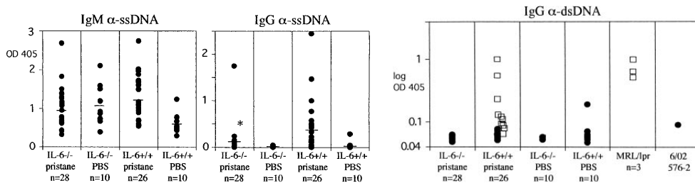
Figure 1. Anti-ssDNA and anti-dsDNA autoantibody levels. (left) Sera from BALB/cAn IL-6 -/- or IL-6 +/+ mice 3 wk after pristane or PBS treatment were tested by ELISA for IgM anti-ssDNA antibodies at a dilution of 1:500. Sera from the same mice 8 mo after treatment were tested by ELISA for IgG anti-ssDNA antibodies. Symbols represent individual animals
