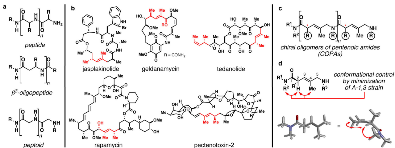
Figure 1. Natural and synthetic oligomers, polyketide-derived natural products, and a polyketide-inspired class of chiral and conformationally rigid synthetic oligomer a , A selection of biological and biopolymer mimetics. b , A selection of polyketide-derived natural products (regions highlighted in red are substituted alkenes that impart conformational rigidification as a result of A1,3 strain). c , General structure of COPAs – chiral oligomers of N -substituted 5-amino-2,4-dialkyl-3-pentenoic amides. d , Structural features that lead to the rigidification of COPA oligomers.
