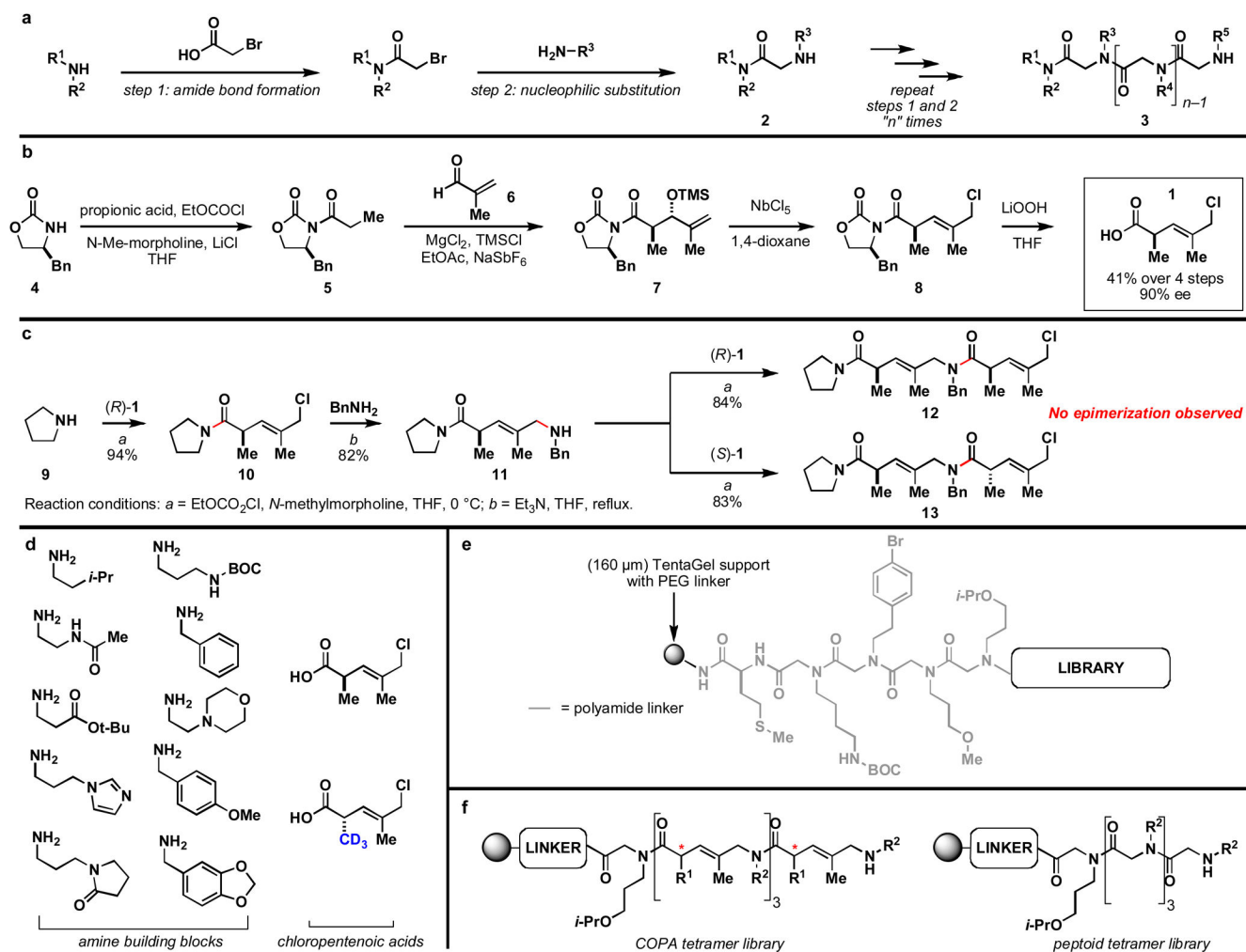
Figure 3. Chemical development of COPA oligomers: From general oligomerization strategy, asymmetric synthesis and library construction
