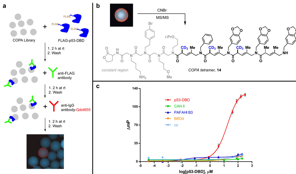
Figure 4. COPA library synthesis, screening, structure elucidation and validation
