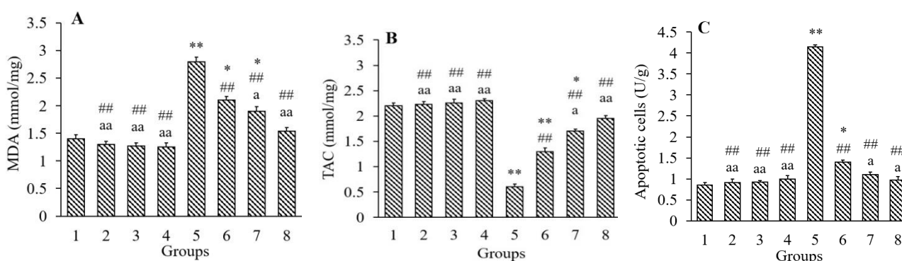
Fig. 3. Outcomes of harmine and cisplatin treatments on the MDA and TAC levels in the kidney tissue and the apoptotic cells in the kidneys of treated-BALB/c mice. Group 1 (control) received normal saline in a dose of 0.09%; groups 2-4 received harmine at 5, 10, 15 mg/kg, respectively; group 5 treated with cisplatin at 5.5 mg/kg; groups 6-8 received cisplatin at 5.5 mg/kg and harmine at 5, 10, and 15 mg/kg, respectively. Values are presented as mean ± SEM; n = 6. * P < 0.05 and ** P < 0.01 indicate significant differences relative to the control group; ## P < 0.01 versus cisplatin group; a P < 0.05 and aa P < 0.01 in comparison with cisplatin + harmine (5 mg/kg) group, respectively. MDA, Malondialdehyde; TAC, total antioxidant capacity.
