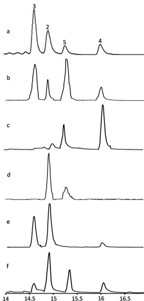
Figure 2 | Total ion chromatograms (TICs) for 10-hydroxygeraniol dehydrogenase (Cr10HGO) catalyzed reactions with (a) 10-hydroxygeraniol and NADP + , (b) 10-oxogeraniol and NADP + , (c) 10-oxogeraniol and NADPH, (d) 10-oxogeraniol and NADPH, (e) 10-hydroxygeraniol and NADP + , (f) 10-hydroxygeraniol and NADPH as substrates. The peaks represent (2) 10-hydroxygeraniol, (3) 10-oxogeraniol, (4) 10-hydroxygeraniol, and (5) 10-oxogeraniol.
