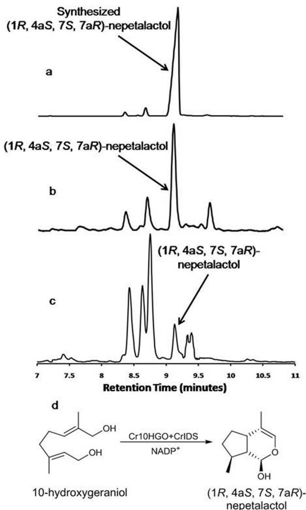
Figure 4 | Comparison of TICs of (a) Synthesized (1 R , 4 aS , 7 S , 7 aR )-nepetalactol, (b) Extract of combined assay of Cr10HGO and CrIDS with 10-hydroxygeraniol and NADP + as substrates, and (c) Extract of CrIDS assay with 10-oxogeraniol and NADPH as substrates. (d) Concerted reaction of Cr10HGO and CrIDS on 10-hydroxygeraniol to form (1 R , 4 aS , 7 S , 7 aR )-nepetalactol.
