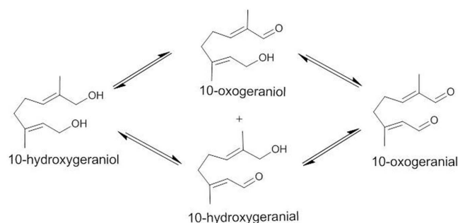
Figure 3 | 10-hydroxygeraniol dehydrogenase (Cr10HGO) catalyzed reaction. NADP + is utilized in the forward reaction, whereas NADPH is utilized in the reverse reactions, generating vice-versa in the process.
