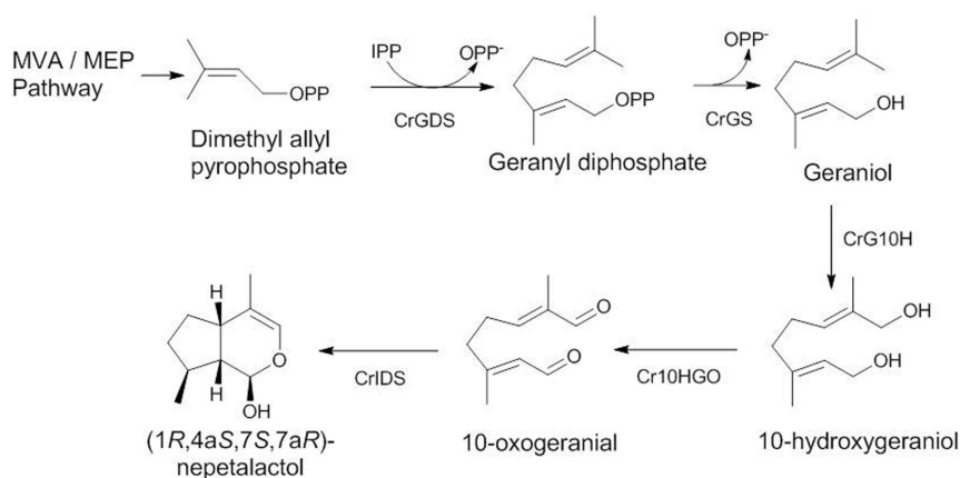
Figure 1 | Iridoid Biosynthetic Pathway cyclizes 10-oxogeraniol into equilibrium mixture of cis-trans-nepetalactol and iridodials. The bicyclic compound, cis-trans-nepetalactol is the key intermediate.
