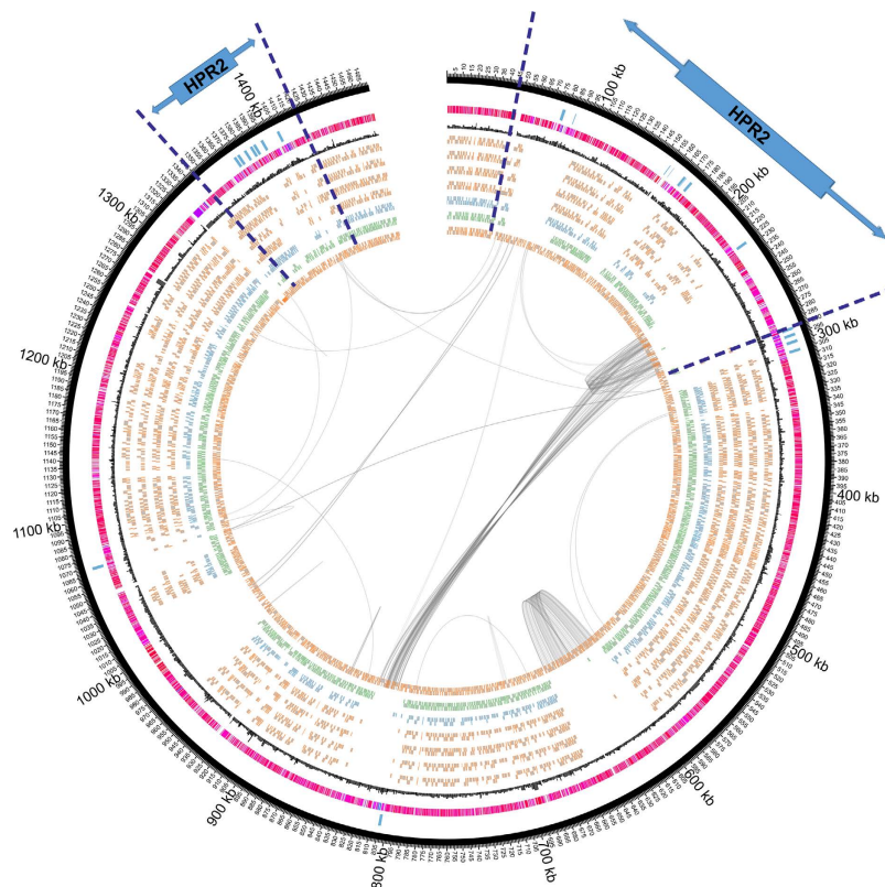
Figure 2. Circular map of Dhc genomes using strain 195 as the reference genome. Genomic coordinates are shown as 100 kbp intervals. From the outer ring, Ring 1 shows the rdhAB genes of strain 195. Ring 2 shows the G + C content of strain 195 shaded in red scale. Ring 3 shows a histogram of codon adaption index or codon usage bias of each gene larger than 200 codons, shaded in greyscale according to their CUB value for emphasis, black indicates highest CUB value of strain 195. Rings 4 to 9 are CDS orthologous to strain 195 in strains GT, CBDB1, VS, BAV1, 11a, and MB, respectively. Curved lines inside circles adjoin repeated elements. The two HPRs of strain 195 are marked with arrows and dashed lines.
