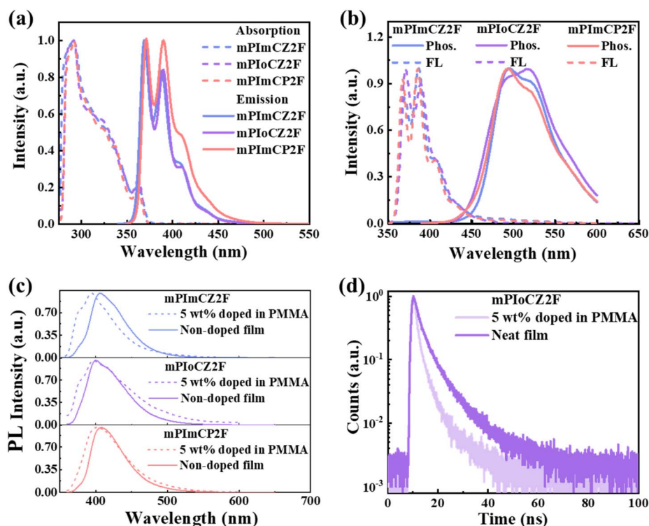
Fig. 3 (a) Absorption and PL spectra of mPImCZ2F, mPloCZ2F, and mPImCP2F in dilute toluene solution ( 10\text{ }\mu\text{M} ) at room temperature. (b) Low-temperature fluorescence (FL) and phosphorescence (Phos.) spectra in ultra-cooled dilute toluene at 77 K. (c) PL spectra of mPImCZ2F, mPloCZ2F, and mPImCP2F in neat films and doped films where they were dispersed in a polymethyl methacrylate (PMMA) matrix at a doping ratio of 5 wt%. (d) Transient PL decay spectra of neat and doped films for mPloCZ2F.
