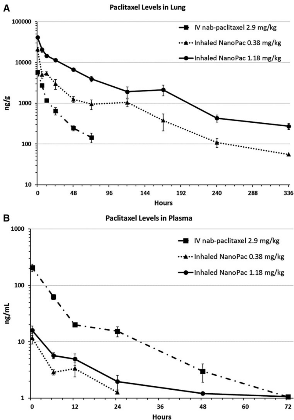
FIG. 3. Postadministration paclitaxel concentration levels (A) in the lung tissue and (B) in the plasma. Male Sprague Dawley rats (6–8 weeks old) were administered paclitaxel on a single occasion in one of three treatment arms ( n = 30 each): inhaled NanoPac in a nose-only exposure at a low dose of 0.38 mg/kg or a high dose of 1.18 mg/kg, or intravenous nab-paclitaxel administered through tail vein injection at 2.9 mg/kg. Three animals from each arm were sacrificed at 0.5, 6, 12, 24, 48, 72, 120, 168, 240, and 336 hours postexposure for lung tissue and plasma collections. Lung tissue (A) and plasma (B) were assayed through ultraperformance liquid chromatography tandem mass spectrometry to quantify paclitaxel concentration as a function of time with a lower level of quantification of 50 ng/g and 1 ng/mL, respectively (mean \pm 1SEM).
