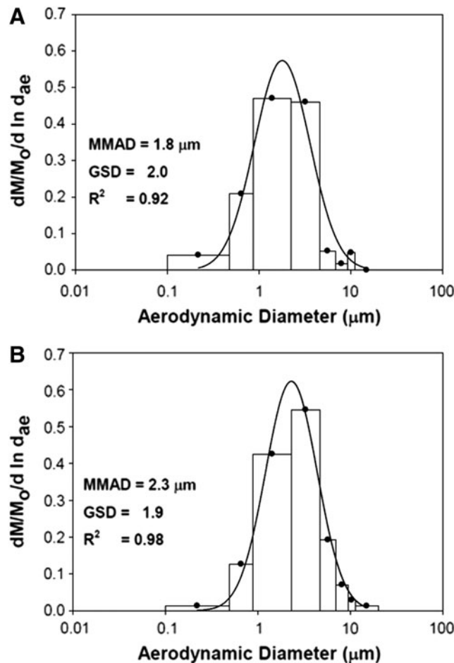
FIG. 2. Mass median aerodynamic size distribution of nebulized (A) 6.0 mg/mL NanoPac suspension and (B) 20.0 mg/mL NanoPac suspension. NanoPac aerosols generated by two Up-Mist compressed air jet nebulizers produced aerosols with MMAD (GSD) of 1.8 (2.0) \mu\text{m} and 2.3 (1.9) \mu\text{m} as measured with the Mercer-style cascade impactor for the 6.0 mg/mL and 20.0 mg/mL suspensions, respectively. MMAD, mass median aerodynamic diameter; GSD, geometric standard deviation; R^2 = coefficient of correlation.
