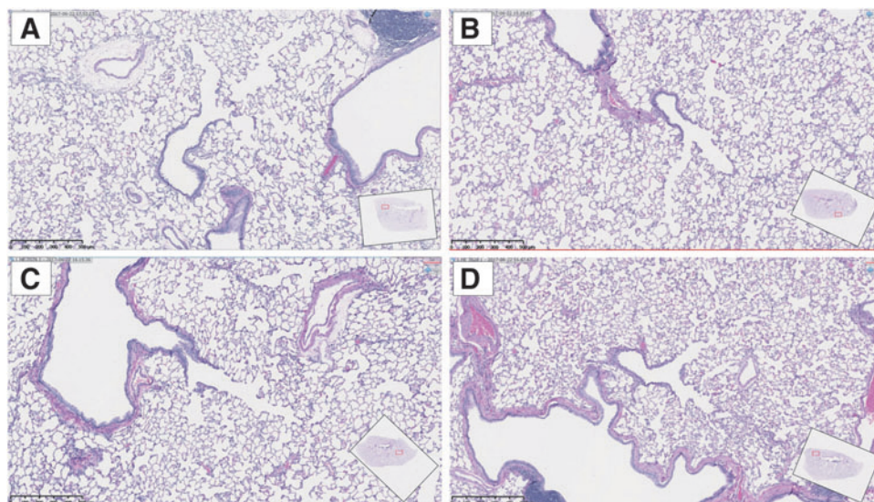
FIG. 4. Histology slides from (A) an untreated rat, (B) a rat treated with intravenous nab-paclitaxel at 2.9 mg/kg, (C) a rat treated with inhaled NanoPac at 0.38 mg/kg, and (D) a rat treated with inhaled NanoPac at 1.18 mg/kg (bar = 500 \mu m). Tissues from fixed left lung lobes of rats sacrificed at the 336-hour time point were processed routinely, paraffin embedded, sectioned at 4 \mu m, mounted, and stained with hematoxylin and eosin for microscopic examination.
