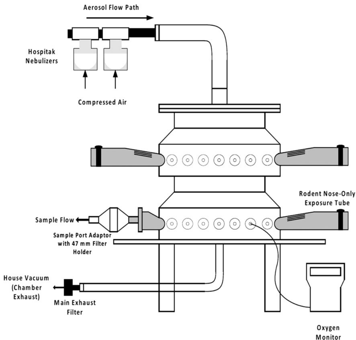
FIG. 1. Schematic of the rodent exposure system for nebulized NanoPac aerosol.
