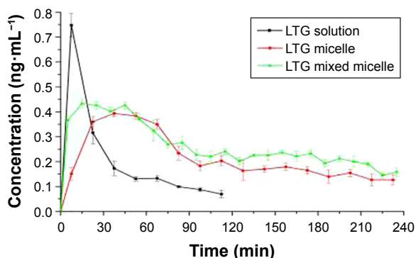
Figure 4 Concentration–time profile of LTG in plasma after nasal administration. Abbreviation: LTG, lamotrigine.
