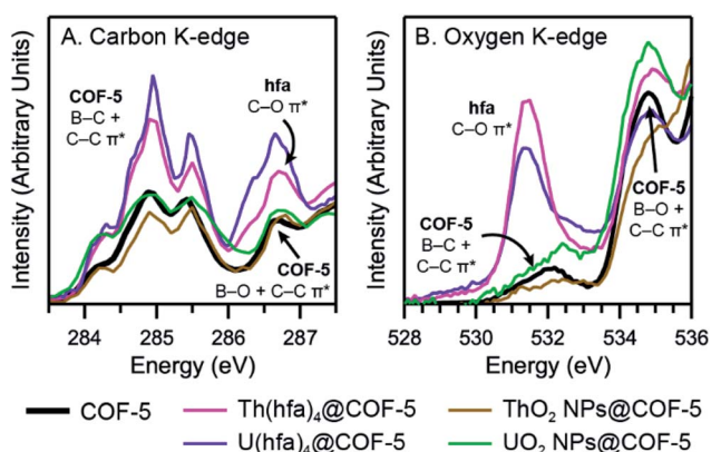
Fig. 6 Plots comparing the C K-edge (A) and O K-edge (B) XAS for \text{Th}(\text{hfa})_4@COF-5 , \text{U}(\text{hfa})_4@COF-5 , \text{ThO}_2 \text{ NPs}@COF-5 , and \text{UO}_2 \text{ NPs}@COF-5 . Feature assignments were derived by comparisons with data reported previously for pure COF-5 and acetylacetone, 124 as well as reference samples \text{Na}(\text{hfa}) , \text{Th}(\text{hfa})_4 , and \text{U}(\text{hfa})_4 (Fig. S10–S12 in the ESI†).
