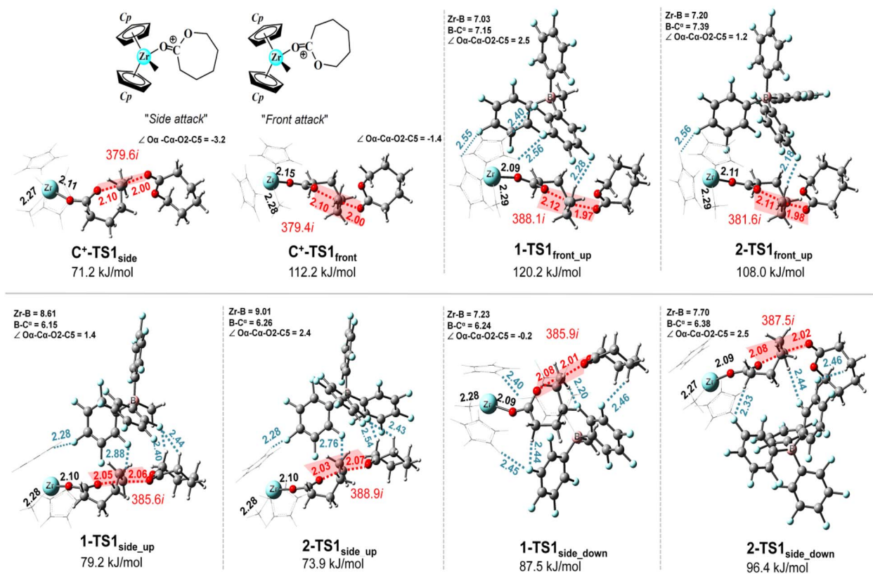
Fig. 2 Optimised transition-state structures (TS1, distances in \text{\AA} ) and their corresponding activation energies (free energies in \text{kJ mol}^{-1} ) relative to R1 for the eight configurations in Fig. 1. Imaginary frequencies (in \text{cm}^{-1} ) are also indicated. A small torsional angle (in deg.) of \text{O}\alpha\text{-C}\alpha\text{-O2-C5} \approx 0\text{--}3 deg. represents a planar alignment of the four-centred transition states. Other planes were also seen for further chain propagations (see ESI † ). Hydrogen bond (F–H) interactions between the cationic species C + and the counteranion are indicated by the dotted line.
