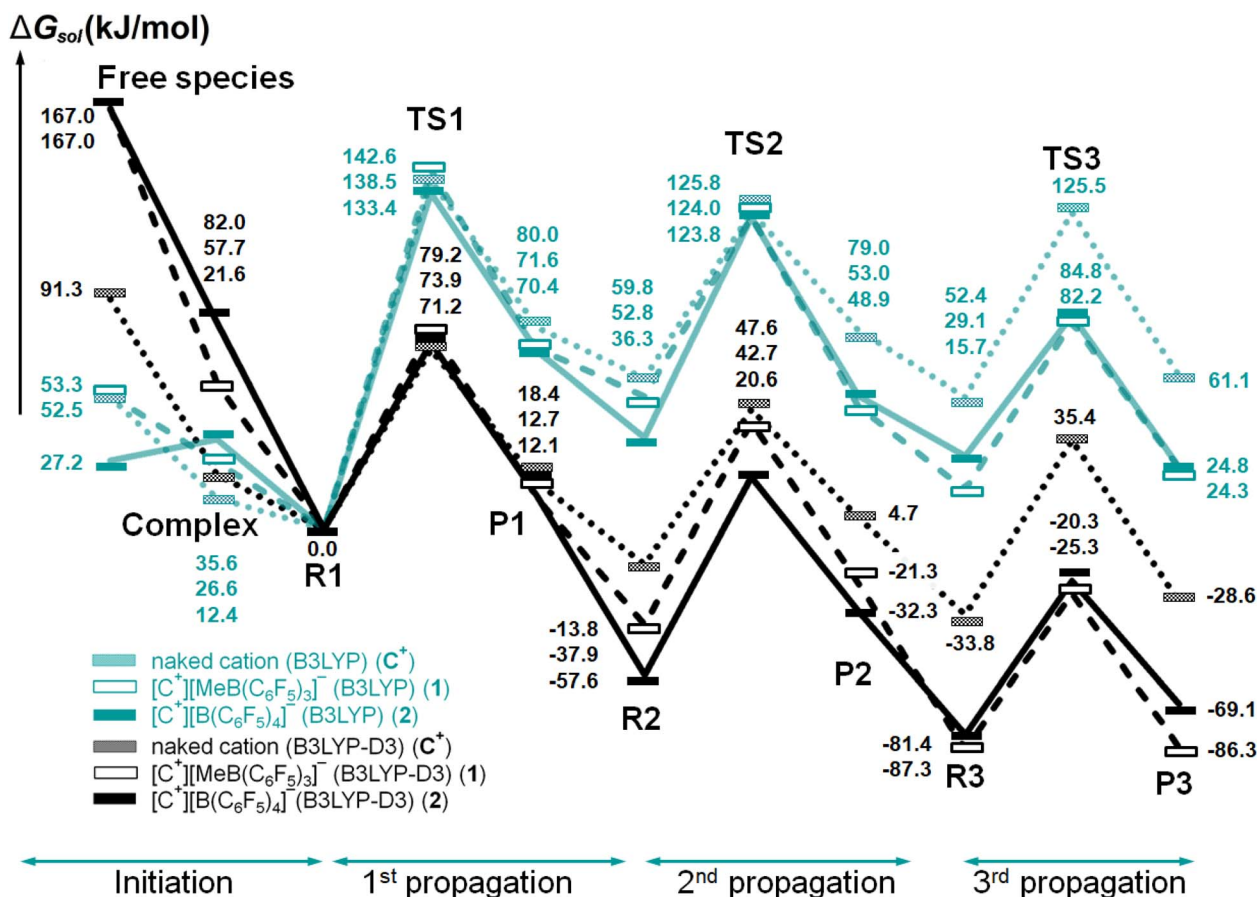
Fig. 3 Gibbs free energy profiles in toluene (shown in black) for the initiation and propagation mechanism of the three catalytic systems (C + , 1, and 2). The uncorrected free energy profiles for the dispersion interaction were also included for comparison (shown in cyan). Relative barrier heights for each of propagation steps were also included in Table 2.
