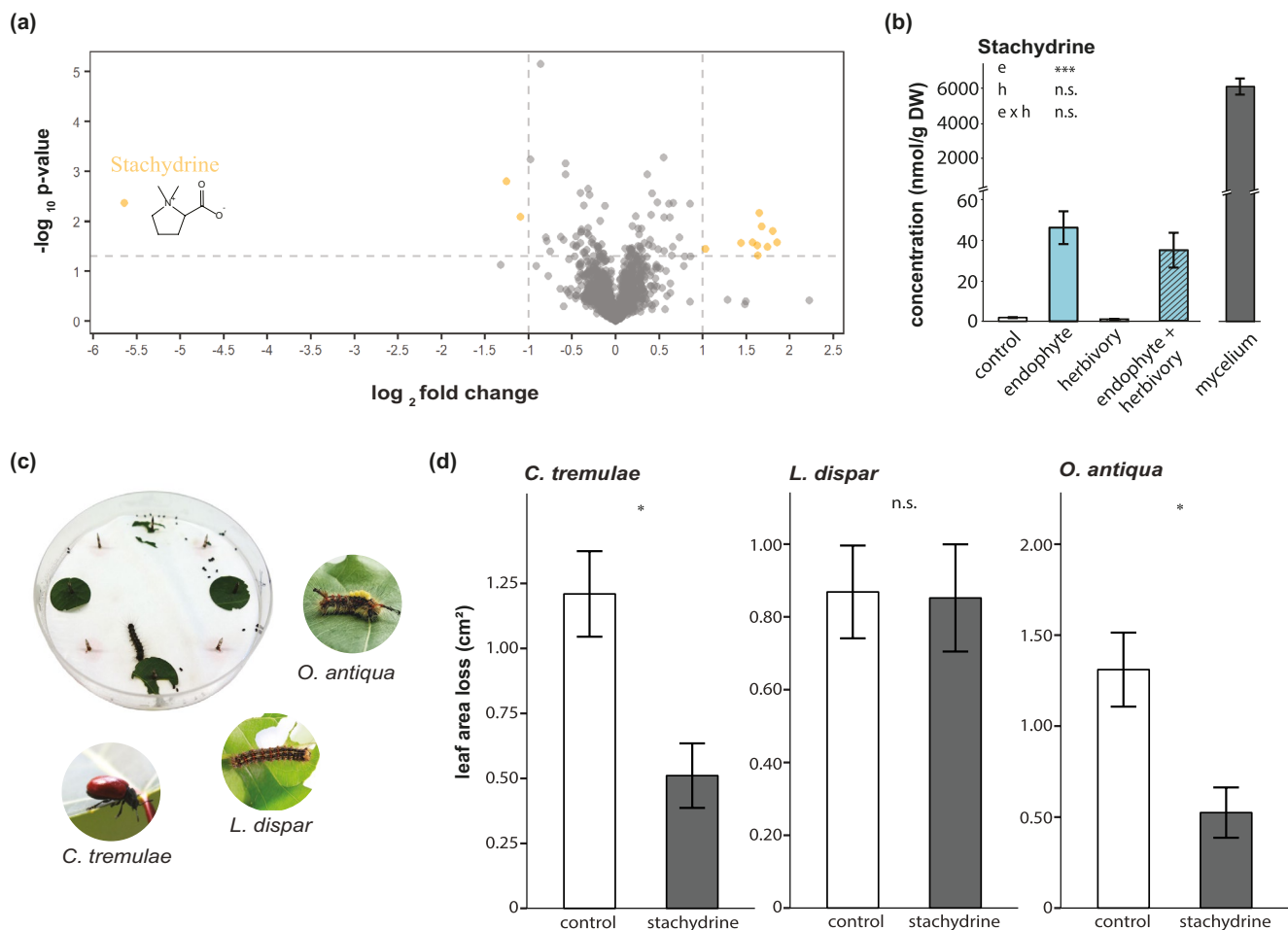
FIGURE 5 | Detection and quantification of the alkaloid stachydrine and its effect on feeding preference of insect herbivores. (a) Volcano plot illustrates metabolite features from leaf tissue inoculated with the endophyte and those of control plants. Features were obtained from an untargeted LC-MS analysis with a QTOF mass spectrometer in positive ionisation mode. Significantly increased or decreased features are highlighted in orange, including the alkaloid stachydrine present in endophyte-inoculated plants. (b) Levels of stachydrine in leaves of black poplar trees under various treatments and in cultured endophyte (mycelium). Trees were either inoculated with endophyte spore solution or a control solution 15 days before the onset of larval feeding, resulting in four treatments: Control , endophyte , herbivory and endophyte + herbivory . After 48 h of herbivory, leaves were harvested. A two-way ANOVA (top left) was used to estimate the effect of endophyte (e), herbivory (h) and the interaction of both (e × h), (* p < 0.05 ; ** p < 0.01 ; *** p < 0.001 ; n.s. = not significant). Mean ± SE are shown ( n = 4 ). The concentration of stachydrine in the mycelium was not included in the statistical analysis. (c) Preference arena containing leaf discs coated either with a stachydrine or control solution. Beetles of C. tremulae and larvae of O. antiqua were allowed to feed for 24 h, L. dispar larvae fed for 48 h. (d) Results of the preference assay for C. tremulae , L. dispar and O. antiqua (left to right). Asterisks indicate significance differences based on related samples Wilcoxon sign rank test ( L. dispar , O. antiqua ,) or a paired t -test ( C. tremulae ) (* p < 0.05 ; ** p < 0.01 ; *** p < 0.001 ; n.s. = not significant). Preference was evaluated as leaf area loss (cm 2 ). Mean ± SE are shown ( n = 20 ).
