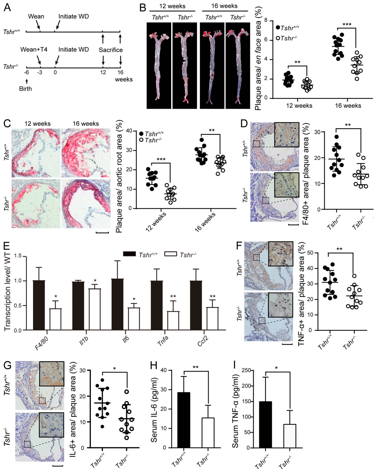
Figure 2. TSHR knockout alleviates vascular inflammation and atherosclerosis in ApoE -/- mice. (A) Schedule of the experiment. Diets of Tshr -/- ApoE -/- mice were supplemented with thyroxine (T4) after weaning. (B and C) Representative Oil Red O–stained whole aorta (B) and aortic root sections (C) of the four groups of mice. (D) F4/80 IHC showing macrophages in aortic root lesions. (E) qPCR analysis of inflammatory marker expression in the aorta. Fold change of the expression level of each marker compared with Tshr +/+ ApoE -/- mice (WT) is displayed. Independent experiments were repeated three times. (F and G) IHC of TNF-α (F) and IL-6 (G) in aortic root sections. (H and I) ELISA of serum IL-6 (H) and TNF-α (I) of the two genotypes. For D–I, data of mice fed WD for 16 wk are shown. Plaque area and stained area of IHC results were measured by Image-Pro Plus software. n = 10–12 (B–D, F, and G), 10–11 (H), or 13–14 (I). Data represent mean ± SD. Scale bars: 200 μm. Differences between two groups were analyzed by t test with Welch’s correction, except for E, which was compared with multiple t tests using Holm–Sidak correction. *, P < 0.05; **, P < 0.01; ***, P < 0.001.
