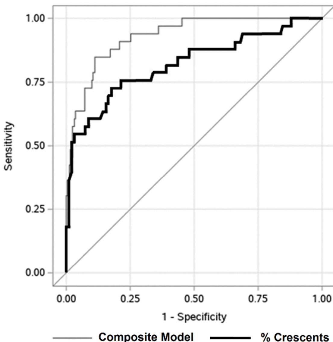
Figure 3. Predicting 1-year renal survival in children with glomerulonephritis with crescents. Receiver operating characteristic curve describing association of percentage of glomerular crescents at biopsy (black line, area under the curve = 0.82) and composite model (gray line, area under the curve = 0.93) with ESKD at one year post biopsy. The AUC for the composite model is significantly higher ( p -value = 0.001). Under the composite model, a predicted probability of 0.14 is the optimal cutoff. When only percent crescents are used to predict end-stage kidney disease (ESKD) at 1-year, 43% is the optimal cutoff.
