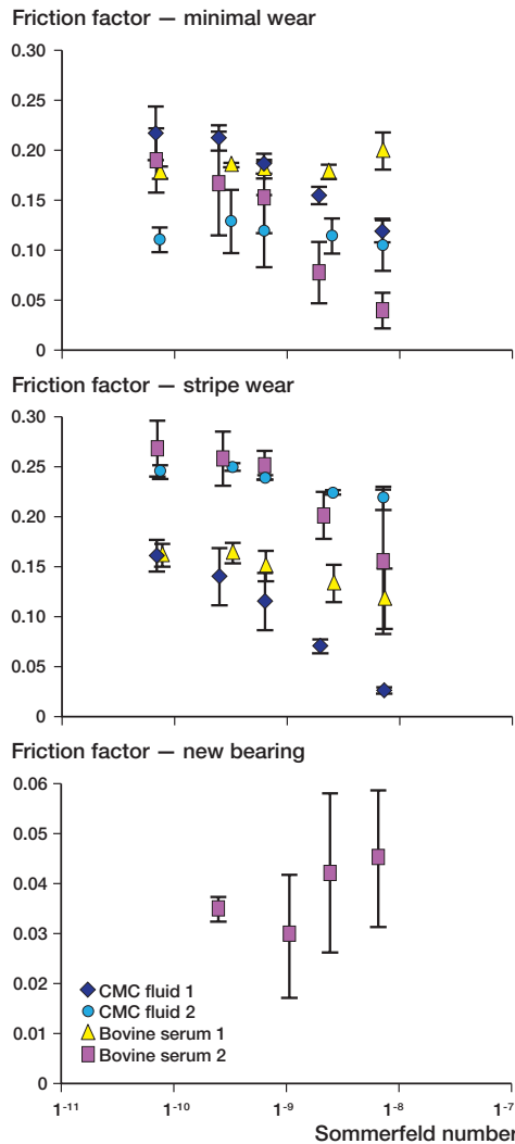
Figure 4. Stribeck plots of bearings with minimal wear and stripe wear, and of a newly manufactured bearing.
