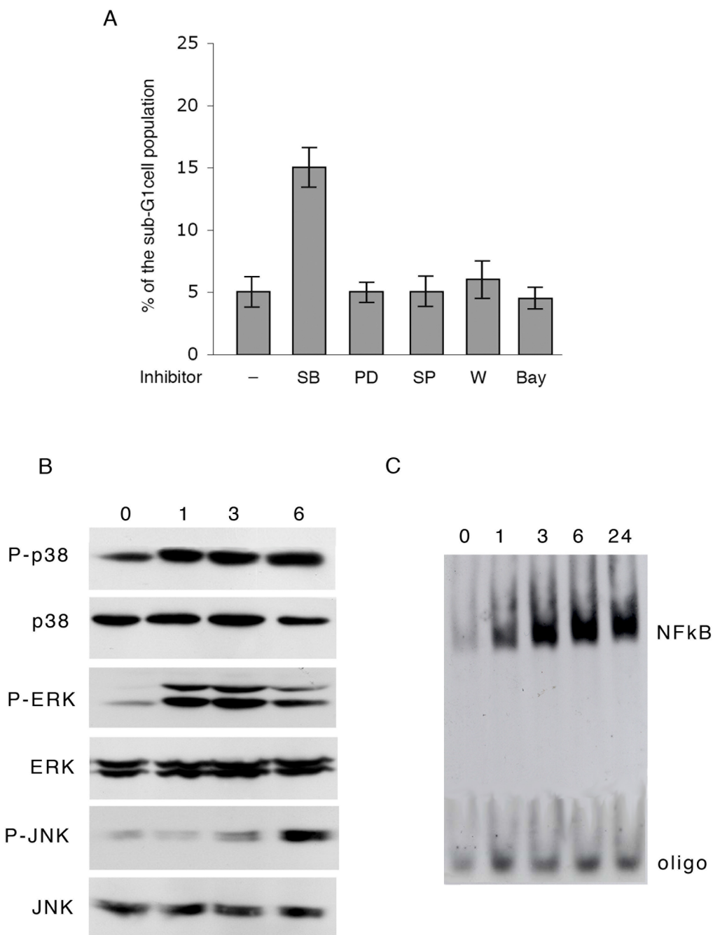
Figure 4 Contribution of signal transduction pathways to cell viability during exposure of Raji cells to EBV lytic cycle activators. (A) Cells were pretreated for 15 min with the specific inhibitors of p38 (SB), ERK (PD), JNK (SP), PI3K (W) or NFkB (Bay) and then exposed to P(BU) 2 , sodium butyrate and TGFβ as described in the Methods. After 48 hours, cells were fixed and PI stained for cytofluorometric determination of sub-G1 events; (B) cells were incubated with P(BU) 2 , sodium butyrate and TGFβ. At the indicated times (hours), cell lysates were prepared and the phosphorylation pattern of p38, ERK and JNK evaluated by Western blot analysis with the specific antibodies for each protein and its phosphorylated (P-) form; (C) cells were treated as in B. At the indicated times, cell extracts were incubated with a consensus NFkB binding site oligonucleotide (oligo) to evaluate NFkB activity by EMSA (see Methods).
