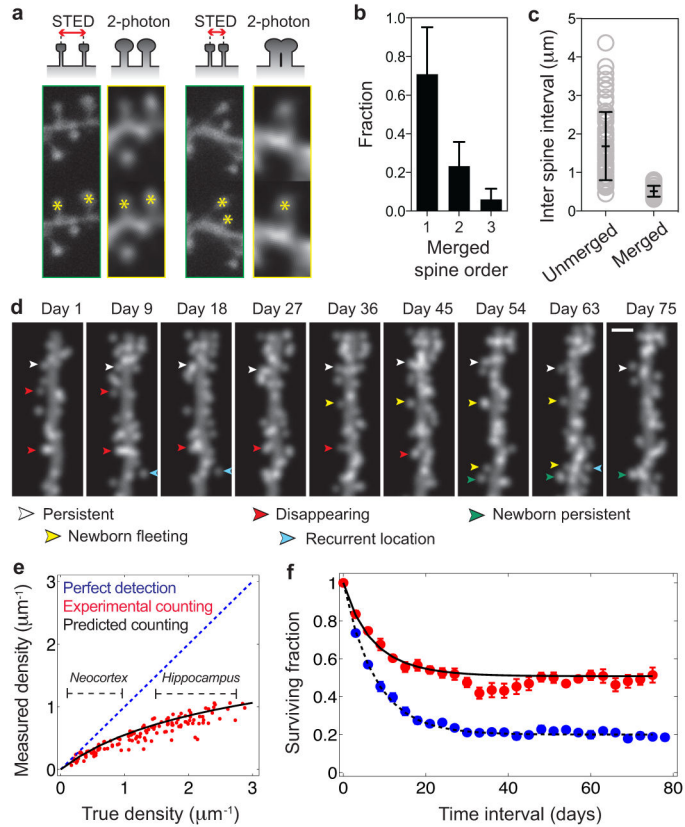
Fig. 2. A simple kinetic model sufficed to describe CA1 pyramidal cell spine dynamics (a) Two-photon microendoscopy and stimulated emission depletion (STED) imaging of the same dendrites in vitro . ( Top row ) two-photon images depict spines closer than the resolution limit as merged entities. ( Bottom ) Asterisks mark example, visually scored spines, showing cases in which nearby spines do ( right ) or do not ( left ) merge. (b) Fraction of spines ( N = 151 total) seen by two-photon imaging, that were one, two or three spines as determined by STED imaging. Error bars: s.d. (c) Separations between adjacent unmerged spines and pairs of spines that appeared merged by two-photon imaging. Open grey circles mark individual results from each of N = 150 spines. Black bars: mean \pm s.d. (d) Example, computer-simulated, time-lapse image sequence, used to quantify how resolution limits impact measured spine densities and dynamics. (e) Computational modeling predicts the underestimation of spine density due to the finite optical resolution. Blue diagonal line: perfect detection of all spines. Black horizontal dashed lines: typical ranges of spine densities on pyramidal cells in neocortex and hippocampus. Red data: results from visually scoring simulated images of dendrites of varying spine densities. Black curve: prediction from the scoring model using 600 nm as the minimum separation between two spines correctly distinguished. (f) Modeling predicts the overestimation of spine stability due to merging of adjacent spines in resolution-limited images. Blue data: Survival fraction values (mean \pm s.e.m.) for actual spine turnover in computer simulations (spine density: 2.56 \mu\text{m}^{-1} ). Red data: Apparent
