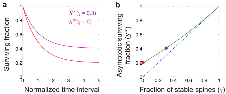
Extended Fig. 4. The asymptotic value of the surviving fraction of spines exceeds the fraction of permanent spines
