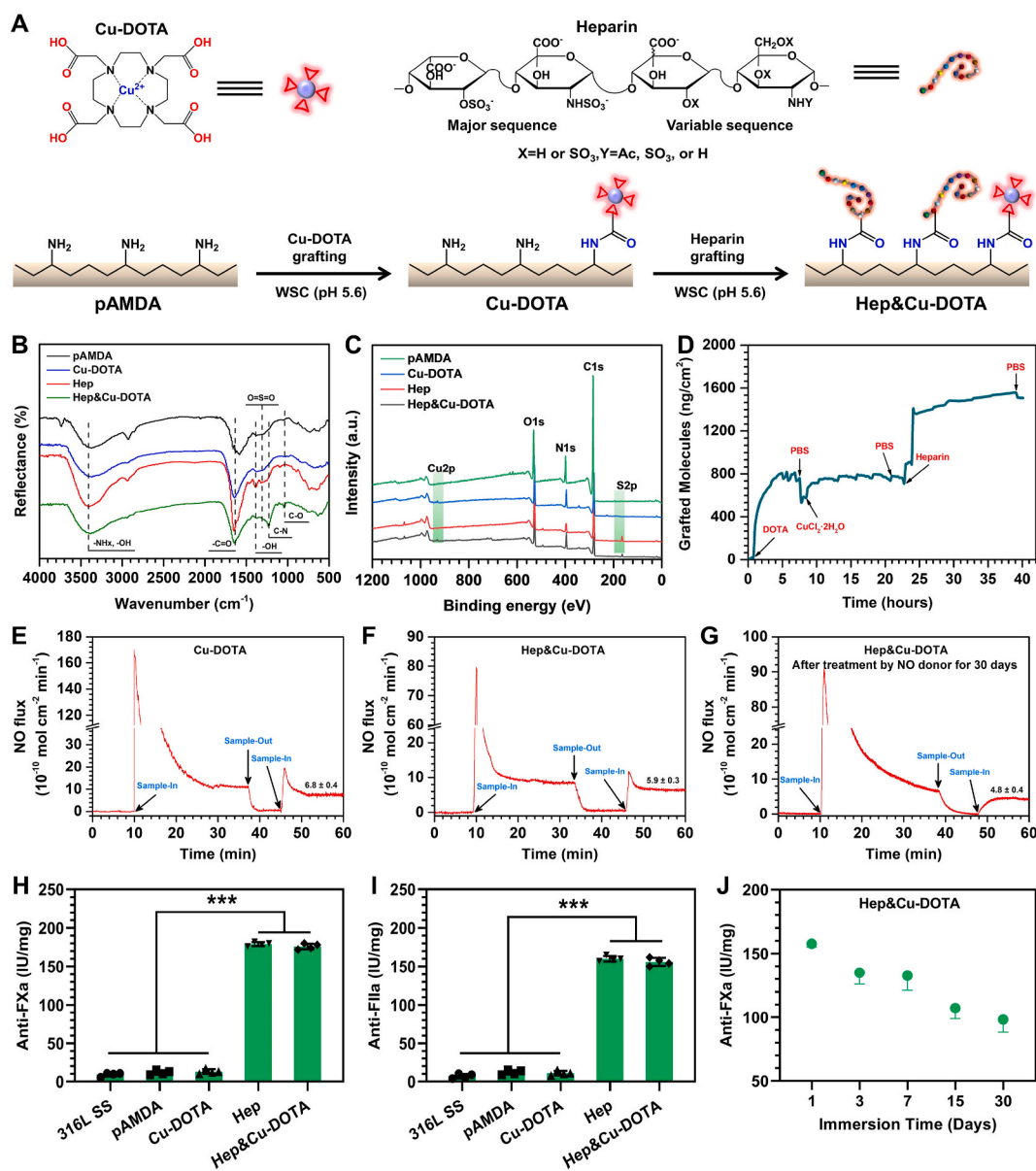
Fig. 2. (A) Cu-DOTA and heparin were stepwisely covalently immobilized on the amine-bearing pAMDA coating based on carbodiimide chemistry. (B) GATR-FTIR spectra and (C) XPS wide-scan survey spectra of the coatings. (D) Real-time monitor of molecule grafting by QCM-D. Real-time release of NO induced by Cu-DOTA (E) and Hep&Cu-DOTA before (F) and after (G) treatment with PBS (pH 7.4) containing NO donor for 30 d. (H, I) Anti-factor Xa and IIa activity of the Hep and Hep&Cu-DOTA coatings and (J) anti-factor Xa activity after treatment with PBS (pH 7.4) for different time intervals. Data are presented as mean ± SD (n = 4) and analyzed using a one-way ANOVA. A p-value less than 0.05 is statistically significant. The symbol *** indicates p < 0.005.
