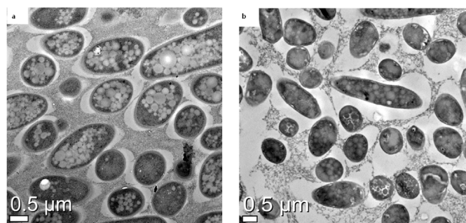
Figure 2 | TEM images of cells collected from the graphite felt (cathode) (a) poised at +0.045 V vs. SHE and (b) under open circuit (no electricity). The phase bright granule within the cell in is clostridial form responsible for solvent production.
