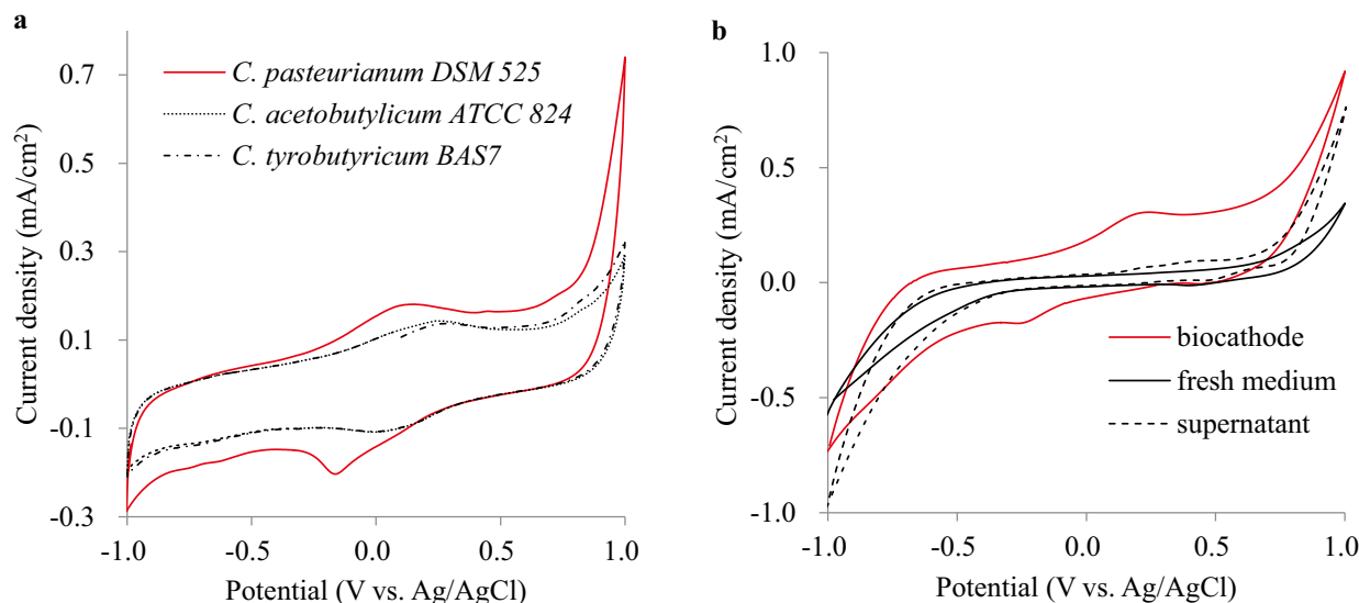
Figure 1 | The cyclic voltammetry (CV) study. (a) The CV of various Clostridium strains. The Ag/AgCl electrode was used as the reference electrode and a glassy carbon electrode as the working electrode. The scan rate was 50 mV/s. Each Clostridium strain was cultured in MP2 medium (glucose 100 mM) and CV was analyzed in a jar separately. Only in C. pasteurianum , the reduction peak was shown at -0.16 V vs. Ag/AgCl ( +0.045 V vs. SHE). (b) The CV of C. pasteurianum cells (biofilm on the cathode and suspended culture) cultivated for 40 hours in the cathode compartment under the potential of -0.16 V vs. Ag/AgCl ( +0.045 V vs. SHE). The scanning rate was 50 mV/s and Ag/AgCl was used as the reference electrode. The biocathode was the working electrode.
