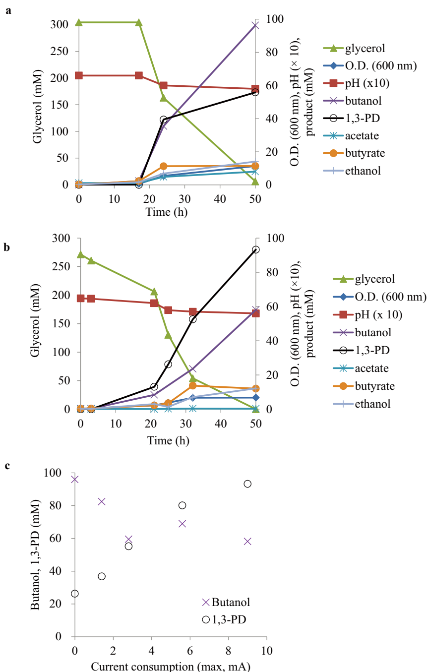
Figure 4 | The glycerol fermentation by C. pasteurianum (a) in control (without electricity) and (b) in bioelectrochemical system poised at +0.045 V vs. SHE with 9 mA current consumption (c) The current consumption-dependent main product shift from butanol to 1,3-PD in glycerol electrofermentation (surface area of electrode: 108 cm 2 ). The current consumption was recorded at the stationary phase with the maximum value and the concentration of product was final concentration when C. pasteurianum completely consumed supplied glycerol.
