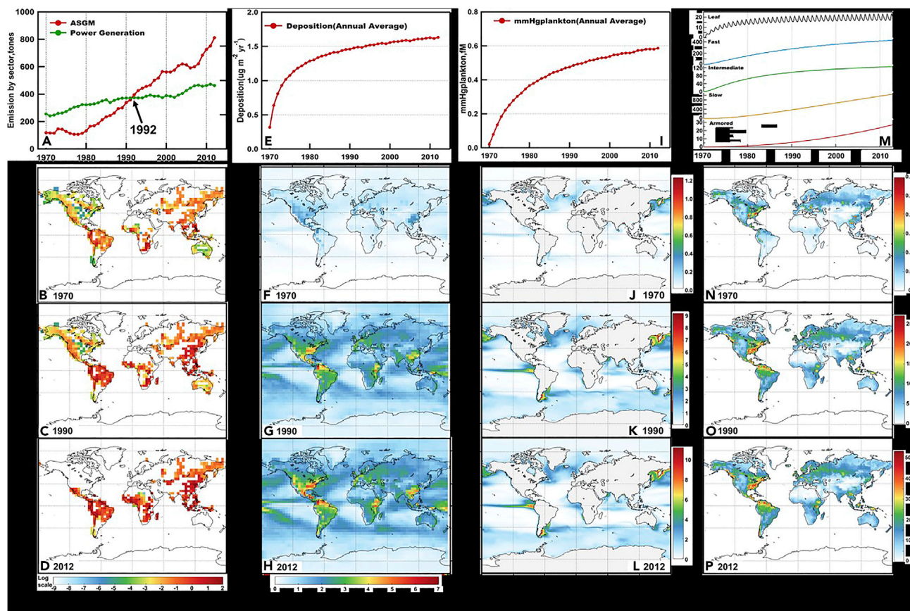
Figure 1. Trends of ASGM Hg emission and its accumulation in the environment
