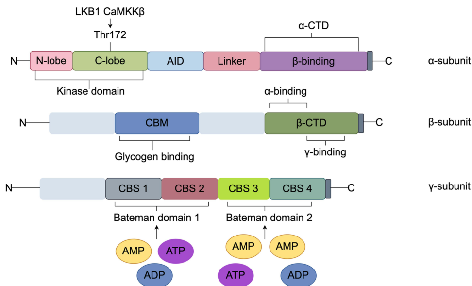
Figure 1 Subunit structure of AMPK.
