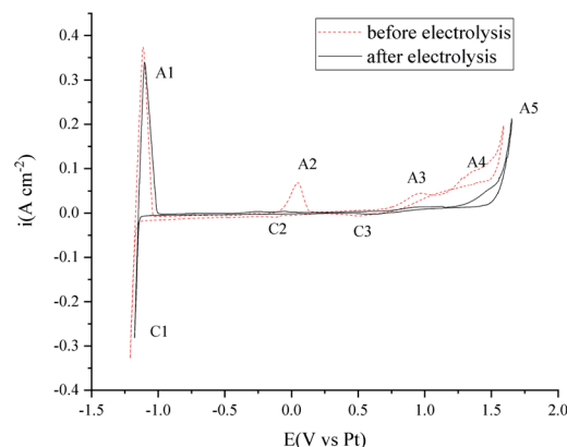
Fig. 7 Cyclic voltammetry investigation in 550 \text{ }^\circ\text{C} MNKC melts before and after 3.5 h electrolysis. Working electrode: W. Reference electrode: Pt. Counter electrode: the nickel vessel. Scan rate: 0.2 \text{ V s}^{-1} .
