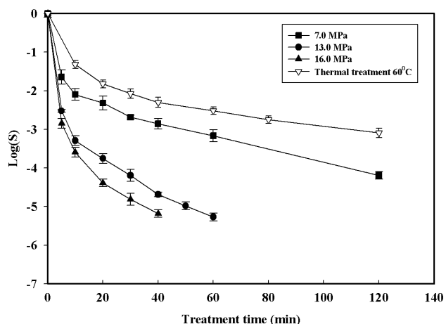
Figure 3 Microbial inactivation of apple juice treated with HPCD as a function of the treatment time for different pressures at 60°C. Values are means of 3 processing runs.
