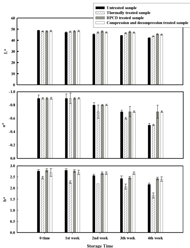
Figure 7 'L*', 'a*' and 'b*' values for untreated, thermally treated, HPCD treated and compression/decompression treated samples as a function of the storage time. The apple juice was treated with heat at 85°C for 60 minutes, with a batch HPCD at 16.0 MPa, 60°C for 50 minutes and with six compression and decompression cycles at 13.0 MPa, 35°C for 10 minutes each.
