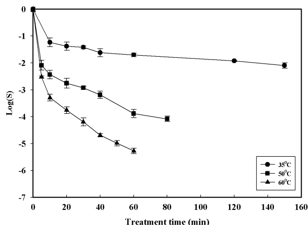
Figure 4 Microbial inactivation of apple juice treated with HPCD as a function of the treatment time for different temperatures at 13.0 MPa. Values are means of 3 processing runs.
