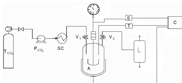
Figure 1 The experimental apparatus: A, vessel with external heater; C, Temperature and magnetic stirrer PID controller; T, thermocouple; S, magnetic stirrer; L, liquid separator. P CO 2 , carbon dioxide pump; SC, cooler system with Peltier effect; T CO 2 , carbon dioxide tank; V 1 , inlet globe valve; V 2 , outlet globe valve.
