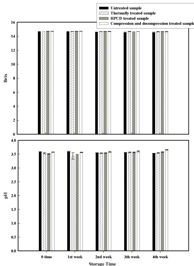
Figure 8 Brix and pH values for untreated, thermal treated, HPCD treated and compression/decompression treated samples as a function of the storage time. The apple juice was thermally treated at 85°C for 60 minutes, with a batch HPCD at 16.0 MPa, 60°C for 50 minutes, and with six compression and decompression cycles at 13.0 MPa, 35°C for 10 minutes each.
