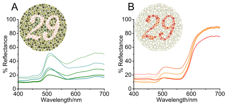
Figure 2. Reflectance spectra of spots corresponding to (A) green (background), and (B) orange (signal) colors of plate 3 of the Ishihara test. This plate contains 5 different shades of green and 5 different shades of orange.
