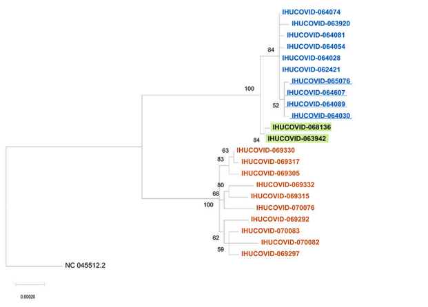
Fig. 2. Schematic of the SARS-CoV-2 Omicron 21L/BA.2-21K/BA.1 recombinant genomes (a, b) and phylogeny reconstruction based on SARS-CoV-2 Omicron 21L/BA.2 and Omicron 21K/BA.1 genomes (c, d).
