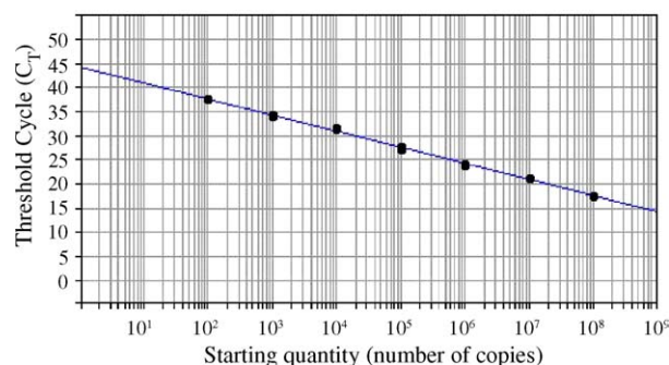
Figure 1 Ten-fold serial dilutions ranging from 10 8 to 10 2 copies of cRNA were tested in duplicate in real-time RT-PCR. A standard curve graph was generated by plotting the C T values on the y-axis and the log of the input amounts on the x-axis. The slope of this standard curve was -3.43 and the correlation coefficient was 0.997.
