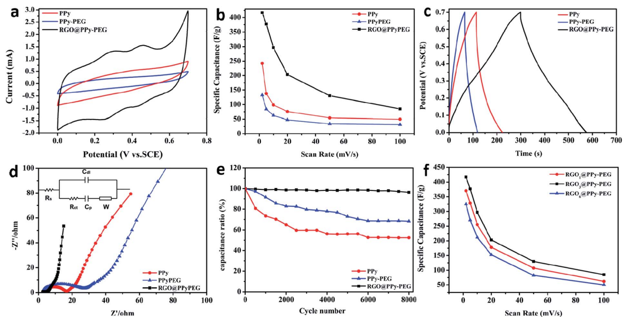
Fig. 4 (a) Comparison of CV curves at scan rate 2 \text{ mV s}^{-1} and (b) plots of specific capacitance versus scan rate for PPy, PPy-PEG and RGO@PPy-PEG foam; (c) GCD curves at current density 1 \text{ A g}^{-1} of PPy, PPy-PEG and RGO@PPy-PEG foam; (d) Nyquist plots and (e) cycling life of PPy, PPy-PEG, RGO@PPy-PEG foam; (f) plots of specific capacitance versus scan rate for RGO 1 @PPy-PEG, RGO 3 @PPy-PEG and RGO 6 @PPy-PEG.
