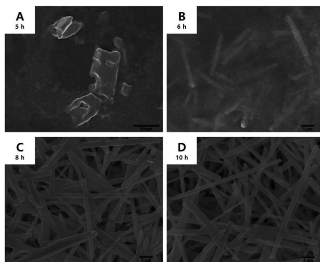
Fig. 1 SEM images of the precipitate over time. (A) Before complete dissolution of tin oxalate; (B) L = 1.85\text{ }\mu\text{m} , R = 0.37\text{ }\mu\text{m} , aspect ratio = 10; (C) L = 6.95 , R = 0.37 , aspect ratio = 37.6; (D) L = 9.25 , R = 0.37 , aspect ratio = 50.
