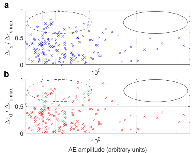
Fig. 5 | Relationship between acoustic emission (AE) amplitude (in log-scale) and local incremental strain at the AE location. a Incremental shear strain, \Delta\epsilon_s (blue crosses), and b incremental dilation, \Delta\epsilon_d (red crosses), each normalised by their respective maximum. The solid black ellipses highlight the lack of large AE events at locations of large strain; indicative of predominantly aseismic deformation. Conversely, the dashed black ellipses highlight locations of large strain which are connected to mostly smaller AE events. Larger AE events are mostly associated with smaller strains.
