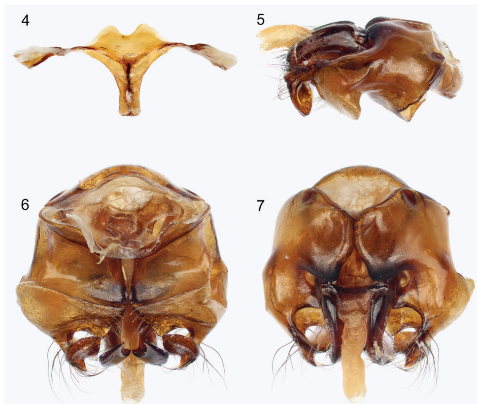
Figures 4–7. Male terminalia of Xylocopa (Koptortosoma) sarawatica Engel, sp. n. 4 Metasomal sternite VII+VIII 5 Genital capsule in profile 6 Genital capsule in ventral view 7 Genital capsule in dorsal view.
