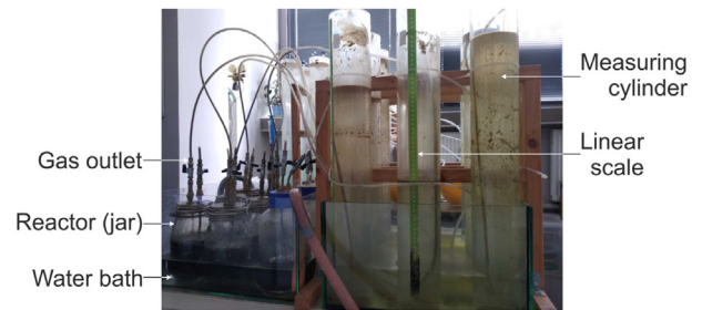
Figure 2. Photo of the experimental setup.
