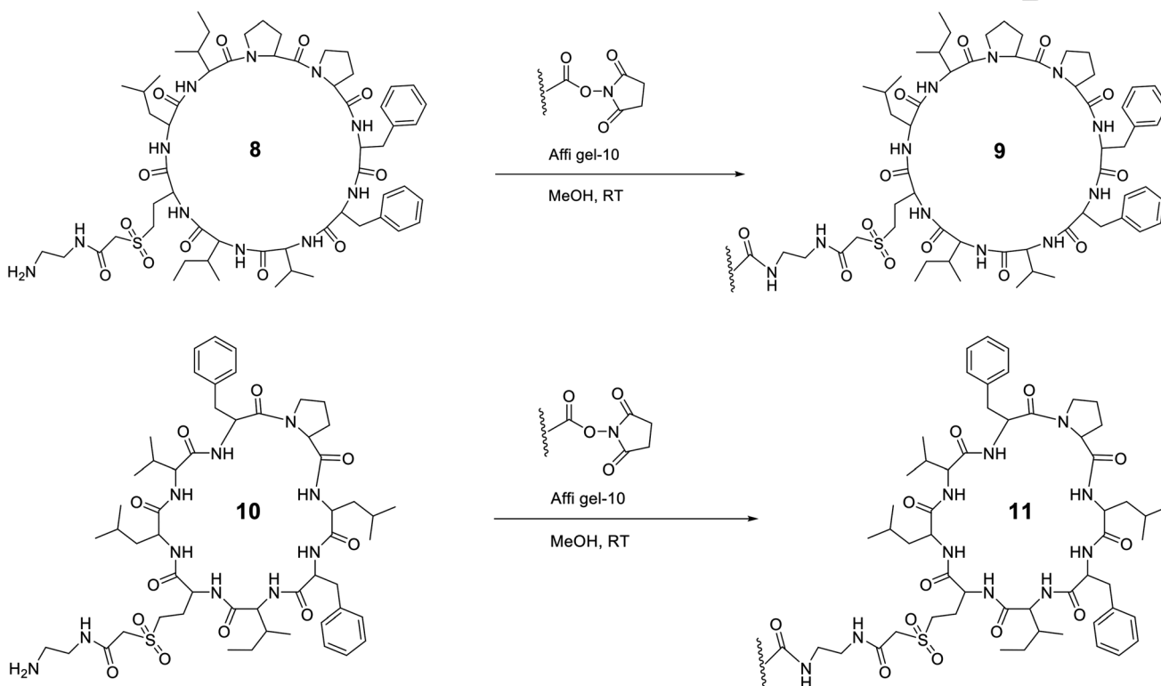
Fig. 1 Chemical structure of LOs 1–7 (A); coupling of 8 and 10 with Affi-Gel 10 (B).
