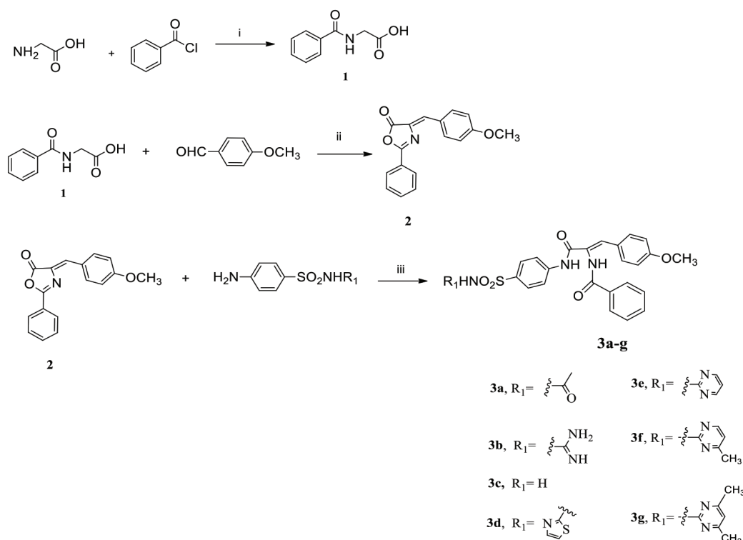
Figure 2. Synthesis of target compounds 3a-g .
