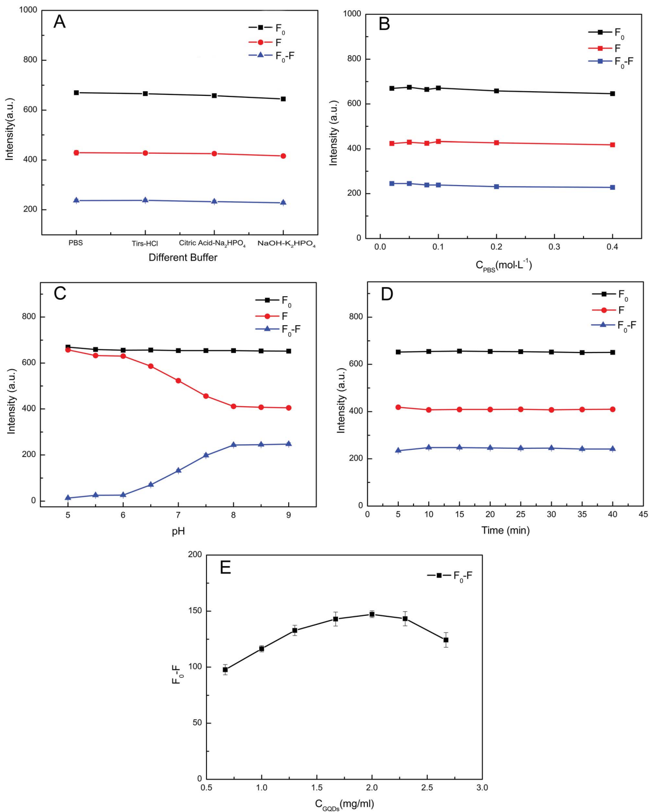
Fig. 8 The influence of different buffer (A) and different concentrations of PBS (B) on GQDs–vanillin reaction system. Effect of pH value on fluorescence intensity of the system (C). The reaction time of GQDs–vanillin reaction system (D). The fluorescence intensity upon different concentrations of GQDs (E).
