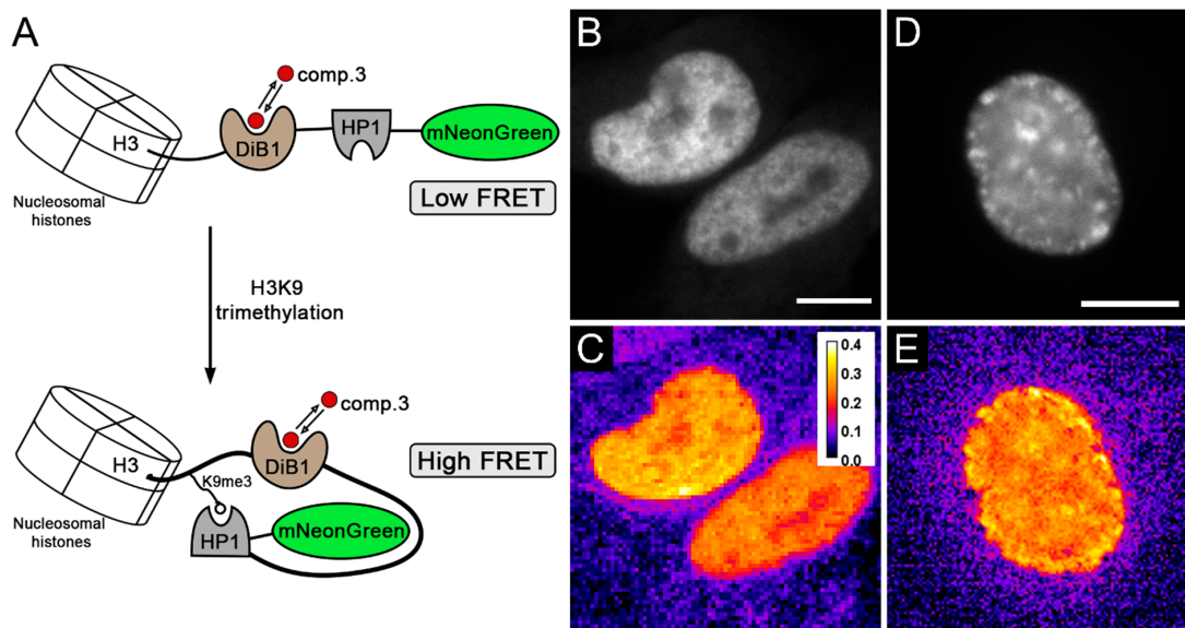
Figure 3. Modified biosensor for H3K9 trimethylation evaluation based on a new FRET pair with the modulated acceptor. (A) Scheme of the new H3K9me3 biosensor and its working mechanism. (B,D) Widefield image of live HeLa Kyoto cells transiently transfected with modified H3K9me3 biosensor construct; scale bar is 5 \mu m. (C,E) Visualization of energy transfer in live HeLa Kyoto cells; pseudocolor indicates FRET efficiency after the addition of compound 3 (3 \mu M). Panels C and E share the same color scale of FRET efficiency.
