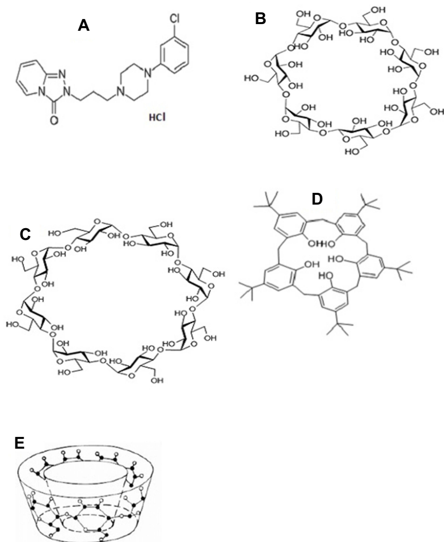
Figure 1 Chemical structures of trazodone (A), \beta -CD (B), \gamma -CD (C), 4 t -BC8 (D), and the toroidal shape (E).
