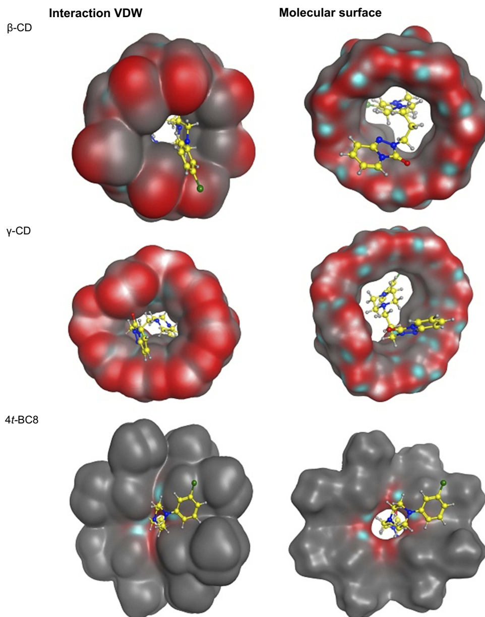
Figure 4 The most stable complex of trazodone with \beta -, \gamma - CD and 4t -BC8 through their cavities.
