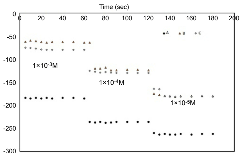
Figure 3 Response time of the proposed (A) \beta -CD, (B) \gamma -CD, (C) 4t-BC8 sensors.
