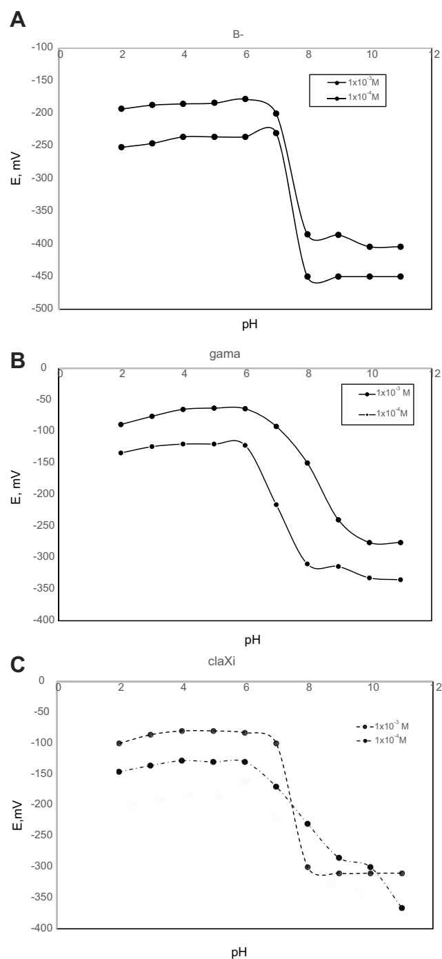
Figure 2 Effect of pH of the proposed sensors (A) \beta -CD, (B) \gamma -CD and (C) 4t-BC8 sensors.
