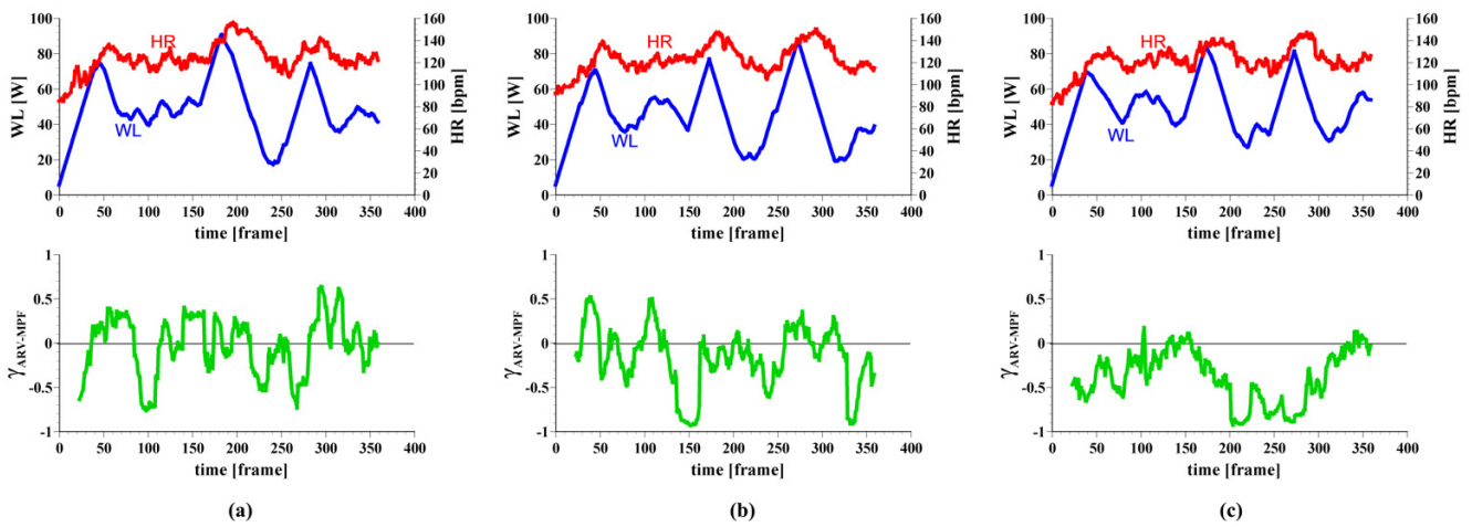
Figure 6 Time-series graphs of different workload patterns for the subject shown in Fig. 5. On the time axis, one frame equals 5 seconds. From top to bottom, workload, heart rate, and \gamma_{ARV-MPF} .
