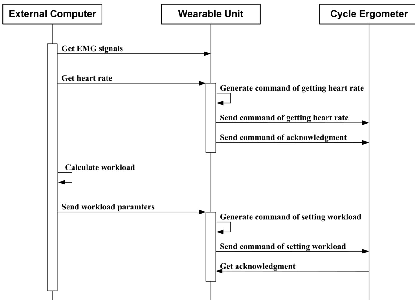
Figure 2 Acquisition-control sequence diagram for controlling the cycle ergometer through the wearable unit with the help of an external computer.
