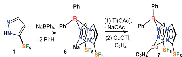
Scheme 2 Synthesis of [Ph 2 B(3-(SF 5 )Pz) 2 ]Cu(C 2 H 4 ).
