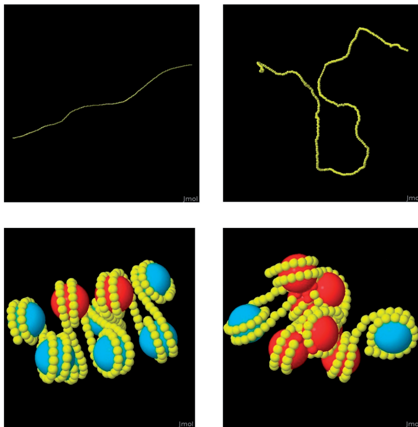
Figure 1. Effect of thermal fluctuations. Thermal fluctuations (left T = 0 \text{ K} ; right T = 298 \text{ K} ) affect both the conformation of free DNA (top images) and the nucleosome arrays (bottom images). For DNA each base pair step allows random thermal motion. In the nucleosome arrays, only the linker DNA allows thermal fluctuations. This can have a significant effect on the overall geometry.
