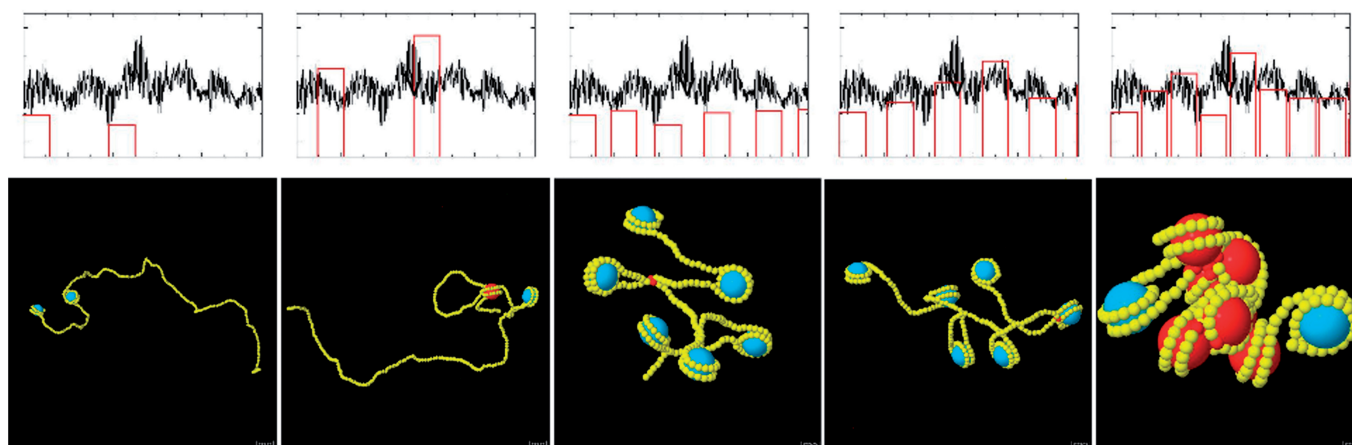
Figure 2. Effect of occupancy. The location of nucleosomes on DNA is a primary determinant of the conformation of the nucleosome array. Here, nucleosome arrays formed with the MMTV sequence and different occupancies are displayed. All have the same energy landscape and a temperature of 298 K. (Left to right) Two nucleosomes automatically placed at the lowest energy positions; two positions specified at high energy locations; 70% occupancy and linker of 20 bp (the default); uniform spacing with a linker of 120 bp; and uniform spacing with a linker of 20 bp.
