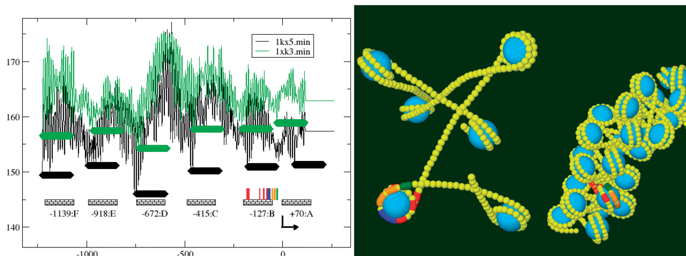
Figure 3. Energy level diagram and conformation of MMTV. (Left) The nucleosome energy level diagram obtained for the MMTV sequence using energy options: 1kx5.min.par and 1kx3.min.par for X_{\text{nuc}} (as indicated), MD-B for K and X_{\text{DNA}} . Energy values are in kcal/mol–nuc. Solid bars indicate the predicted nucleosome footprints and have been shifted so that the transcription start site corresponds to position 0, as indicated by the arrow. Also included are the known positions of nucleosomes A–F, indicated as tiled boxes, glucocorticoid response elements (red), NF1 (blue) and Oct (orange) binding sites, and the TATA box (green). (Middle) The 3 D structure of the MMTV associated with this energy landscape for a temperature of 0 K. Yellow spheres represent 5 bp. Histone cores as light blue spheres. Here, the glucocorticoid response elements are red, NF1 binding sites are blue, octamer binding sites are orange, and the TATA box is green. Nucleosome A is in the bottom right and B is in the bottom left. (Right) Five tandem repeats of the MMTV with a uniform spacing ( n_{\text{lk}} = 30 ) of nucleosomes, and temperature 0 K. The first repeat is shifted to achieve the lowest energies. The bend only arises from deformations present in the linker DNA.
