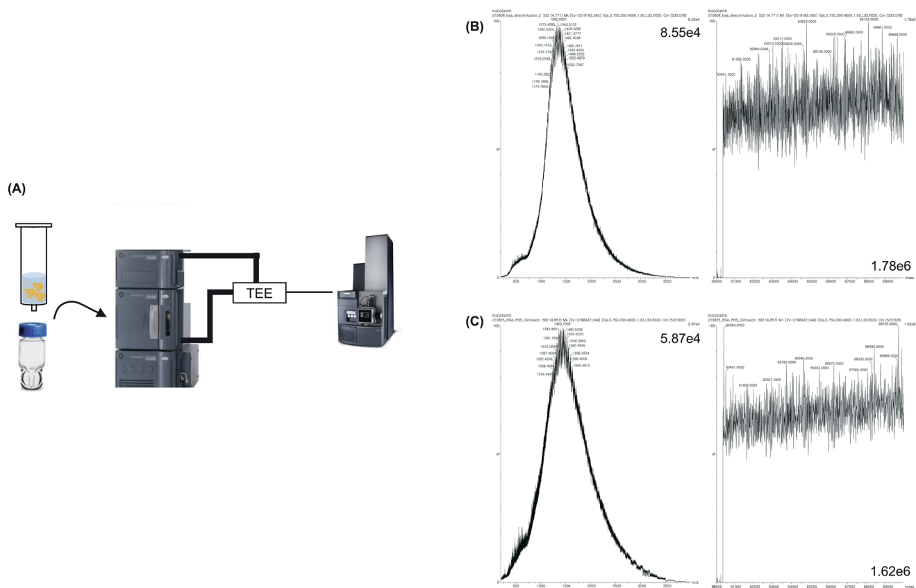
Fig. 2 BSA intact protein MS analysis without desalting. (A) Schematic diagram of the direct infusion without desalting, (B) MS spectrum and deconvolution results of BSA sample dissolved in 1 M PBS with 0.1% formic acid, (C) MS spectrum and deconvolution results of BSA sample dissolved in 1 M PBS.
