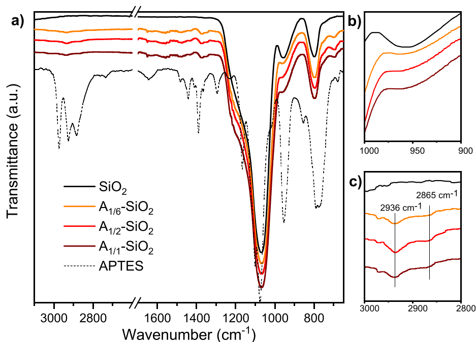
Figure 1. (a) FTIR spectra of A_X -SiO 2 compared with bare SiO 2 and pure APTES. (b) Magnification of the ranges 900–1000 cm -1 and (c) 2800–3000 cm -1 .
