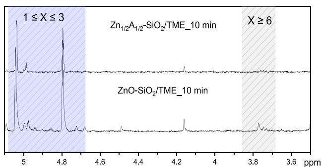
Figure 6. ^1H NMR spectra (range, 3.5–5.1 ppm) of Zn_{1/2}A_{1/2}-SiO_2/TME and ZnO-SiO_2/TME after 10 min of reaction time.
