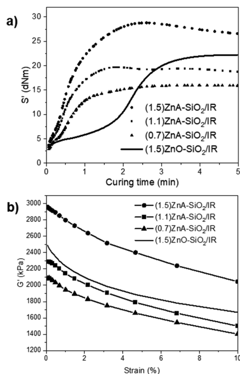
Figure 5. Comparison of the vulcanization curves (a) and of the elastic modulus G' (b, 0–10% strain) measured for SiO_2 /IR NCs cured with Zn_yA_x-SiO_2 at different Zn contents: (1.5)ZnA- SiO_2 /IR (circles), (1.1)ZnA- SiO_2 /IR (squares), and (0.7)ZnA- SiO_2 /IR (triangles). Vulcanization and G' curves of (1.5)ZnO- SiO_2 /IR NCs (solid line) are also reported in (a) and (b), respectively, as a reference sample.
