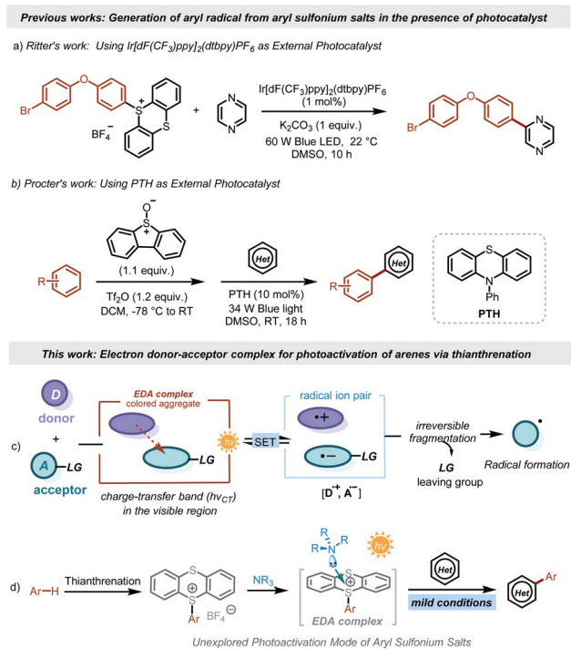
Scheme 1 Photocatalytic arylation of aryl sulfonium salts.
