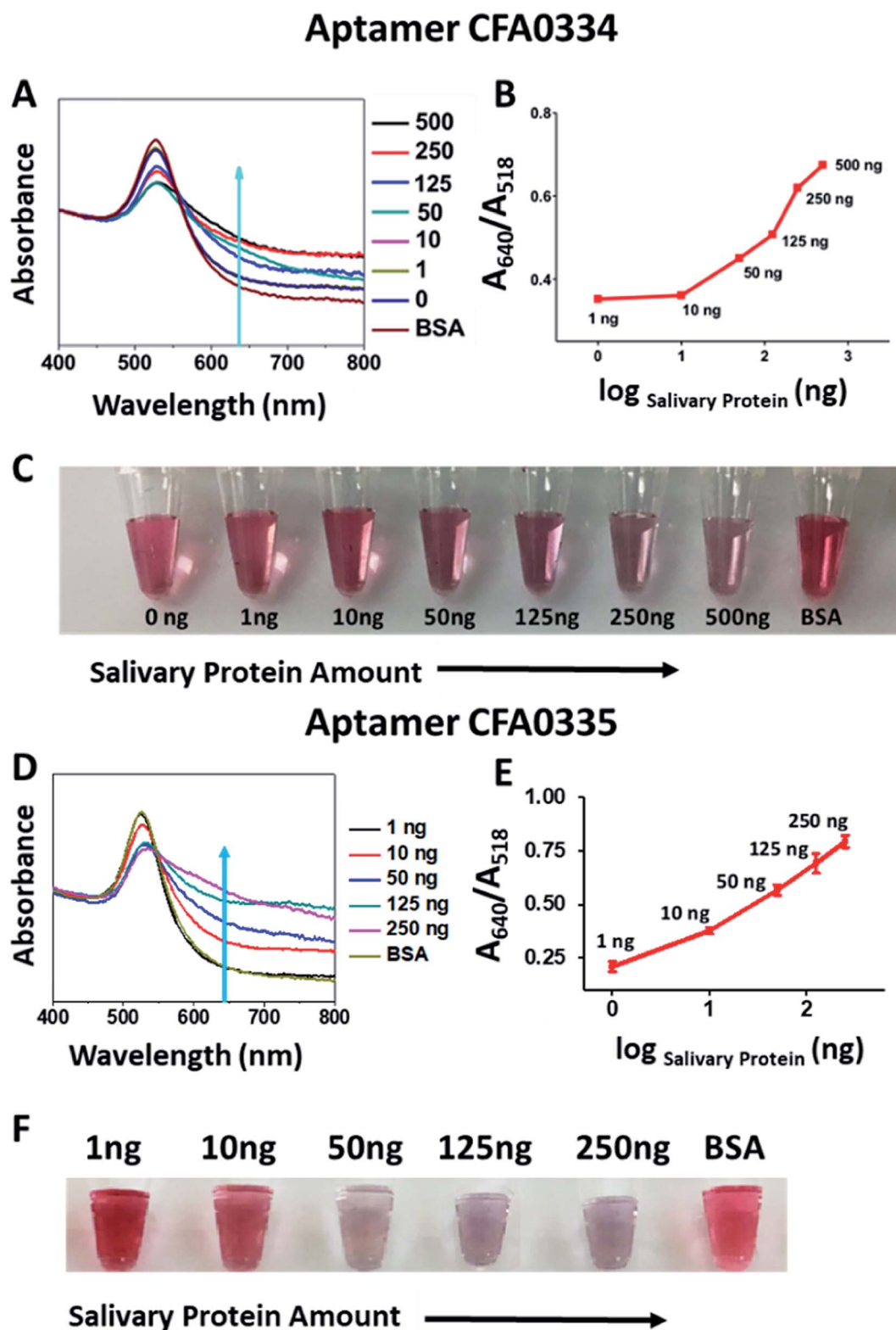
Fig. 4 Sucrose-capped Apt–AuNPs detection of Ae. aegypti SGE. (A) UV-visible spectroscopy, (B) A_{640}/A_{518} ratios and (C) corresponding digital image of the CFA0334-derived Apt–SAuNPs in the presence of SGE show a dose dependent increase in particle aggregation with detection as low as 50 ng Ae. aegypti SGE. BSA used as control. Corresponding (D) UV-visible spectroscopy, (E) A_{640}/A_{518} ratios and (F) corresponding digital image of CFA0335-derived Apt–SAuNPs showing a dose dependent increase in aggregation in response to SGE as low as 10 ng. BSA used as control.
