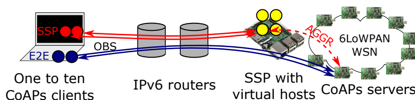
Figure 8. Evaluation setup: a variable number of CoAPs clients observes one of two resources on either the virtual host (SSP) or the sensor node (E2E).
