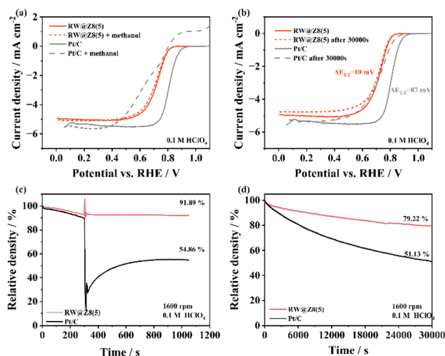
Fig. 6 (a) LSV curves of RW@Z8(5) and Pt/C in O 2 -saturated 0.1 M HClO 4 solution at a rotation speed of 1600 rpm with/without 1 M methanol; (b) LSV curves of RW@Z8(5) and Pt/C before and after 30 000 s durability measurement in O 2 -saturated 0.1 M HClO 4 solution at a rotation speed of 1600 rpm; (c) chronoamperometric responses of RW@Z8(5) and Pt/C at 0.6 V in O 2 -saturated 0.1 M HClO 4 solution at a rotating rate of 1600 rpm with 1 M methanol added at 300 s; (d) Current–time ( i - t ) durability measurement for RW@Z8(5) and Pt/C at 0.6 V in O 2 -saturated 0.1 M HClO 4 solution with slight bubbling at a rotating rate of 1600 rpm.
