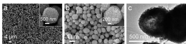
Fig. 2 (a) FESEM image of SnO 2 -UF microspheres precursor, (b) FESEM and (c) TEM image of pure SnO 2 hollow spheres.
