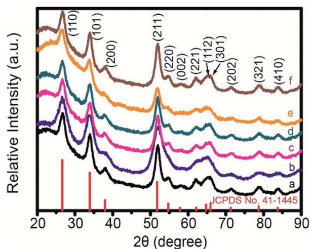
Fig. 4 XRD pattern of Pd-loaded SnO 2 hollow spheres with Pd amount of (a) pure, (b) 0.1 wt%, (c) 0.2 wt%, (d) 0.5 wt%, (e) 1 wt% and (f) 2 wt%, respectively.
