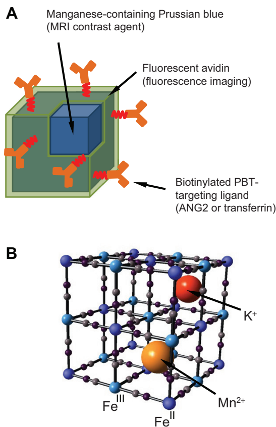
Figure 1 Manganese-containing Prussian blue nanoparticles for imaging of PBTs. Notes: (A) Schematic representation of manganese-containing Prussian blue nanoparticles comprised of an inorganic core that provides MRI contrast and a biofunctionalized shell consisting of fluorescently-labeled avidin and biotinylated PBT-targeting ligands. (B) Schematic representation of the Prussian blue lattice (ball and stick) containing interstitial Mn^{2+} and K^+ ions. Abbreviations: ANG2, anti-neuron-gial antigen 2; MRI, magnetic resonance imaging; PBT, pediatric brain tumor.
