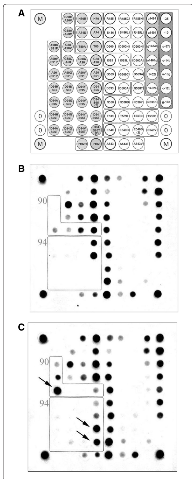
Figure 1 Analysis of Mycobacterium tuberculosis drug susceptibility by hybridisation on a biochip. (A) The scheme of the biochip for hybridisation. The subgroups are depicted as boxes. Each subgroup corresponds to a single variable amino acid position or variable nucleotide. One gel element within each subgroup contained an oligonucleotide matching the wild-type sequence (bold circles). (B) Hybridisation of a wild-type DNA sample on the biochip. (C) Hybridisation of a DNA sample containing the following mutations indicated by arrows: gyrA (S91P, TCG > CCG) and gyrA (S95T, AGC > ACC).
