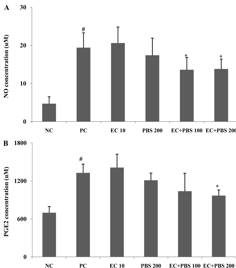
Figure 3. Effects of EC, PBS and EC+PBS on concentration of nitric oxide (A) and prostaglandin E2 (B) The data were expressed as mean \pm SD. The data were expressed as mean \pm SD. NC: Normal control, PC: MIA alone, EC 10: Egg white-chalcanthite 10 mg/kg b.w, PBS 200: Purple bamboo salt 200 mg/kg b.w, EC-PBS 100: EC+PBS 100 mg/kg b.w, EC+PBS 200: EC+PBS 200 mg/kg b.w. #, significantly different from NC at P < 0.05 . *, significantly different from PC at P < 0.05 .
