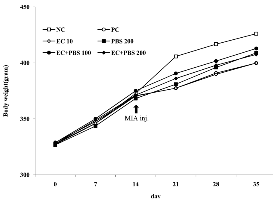
Figure 2. Effect of EC, PBS and EC+PBS on the body weight in rats. The data were expressed as mean \pm SD. NC: normal control, PC: MIA alone, EC 10: egg white-chalcanthite 10 mg/kg b.w, PBS 200: purple bamboo salt 200 mg/kg b.w, EC+PBS 100: EC+PBS 100 mg/kg b.w, EC+PBS 200: EC+PBS 200 mg/kg b.w.
